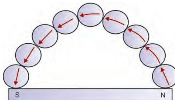
Fig. 1.45: Magnetic line of force
