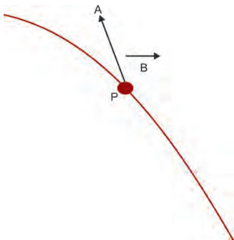
Fig. 1.44: Tangent to a magnetic line of force
