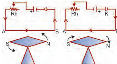
Fig. 1.25: Magnetic effects of electric current
