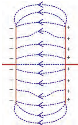
Fig. 4.9: Distance too small
