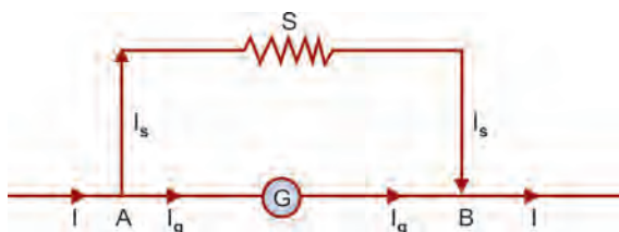
Fig. 1.36: Shunt
