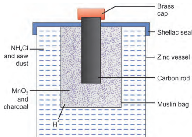
Fig. 1.22: Dry cell
