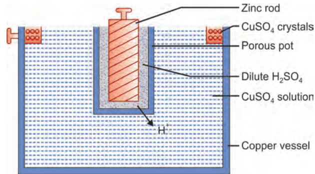
Fig. 1.20: Daniel cell
