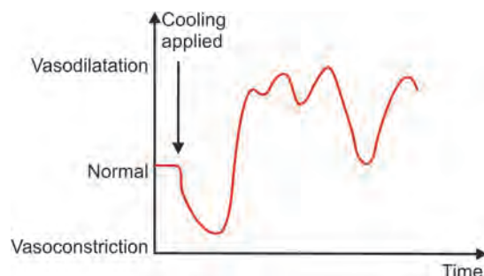
Fig. 9.3: Lewis-Hunting reaction
