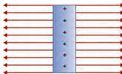
Fig. 1.7: Lines of force due to large sheet
