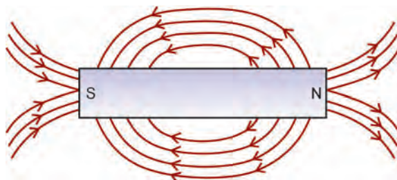
Fig. 1.46: Direction of magnetic lines of force
