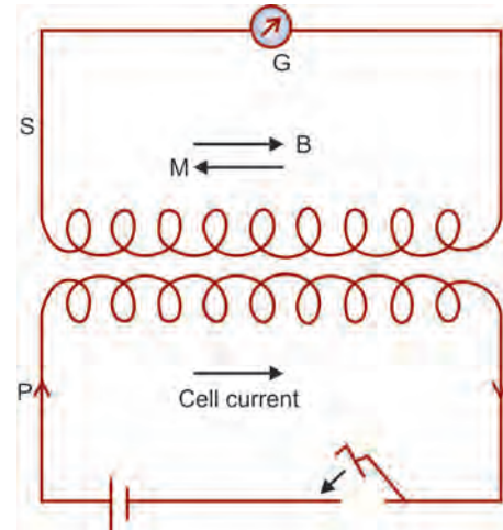
Fig.1.58: Mutual induction
