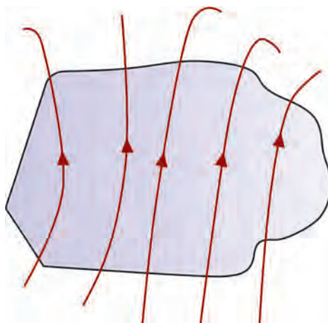
Fig. 1.49: Magnetic field lines
