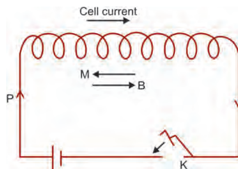
Fig. 1.57: Self induction
